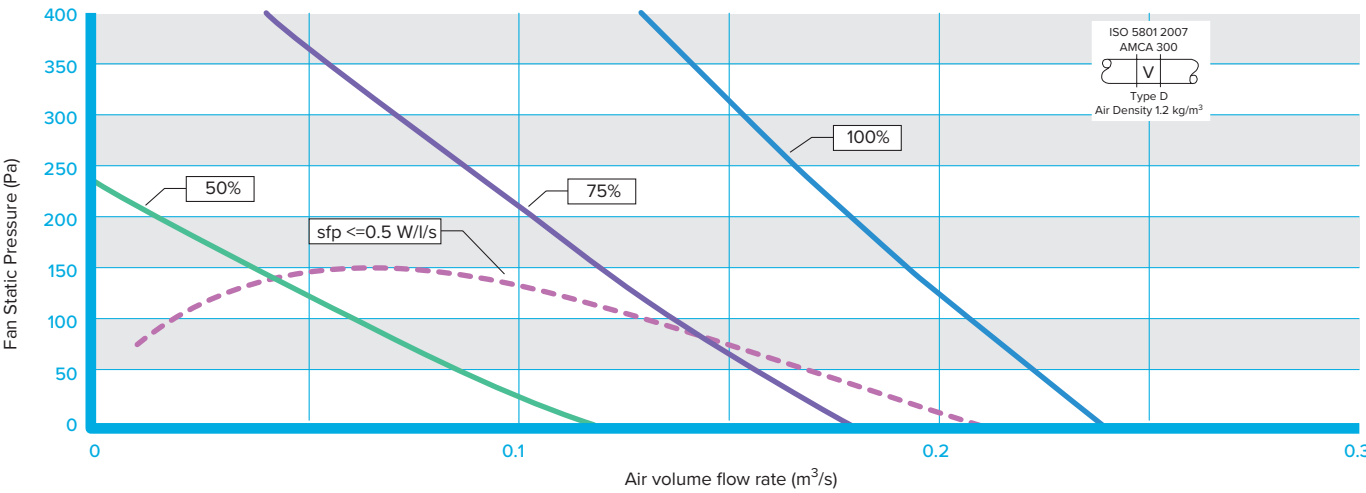
EXTRACT FAN SIZE DE2H - PERFORMANCE
