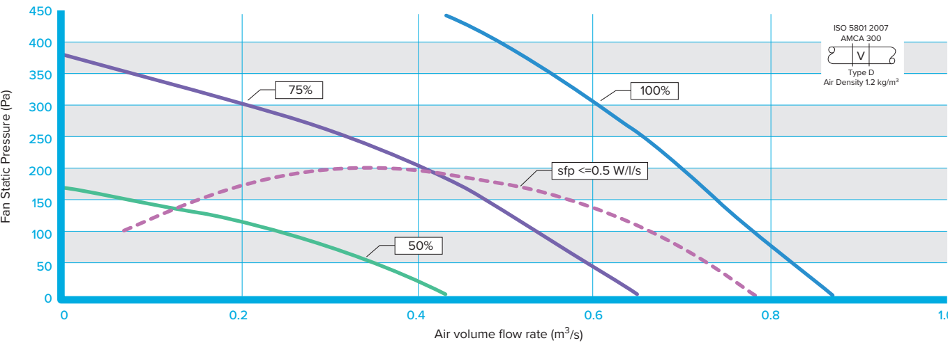
EXTRACT FAN SIZE DE6 - PERFORMANCE
