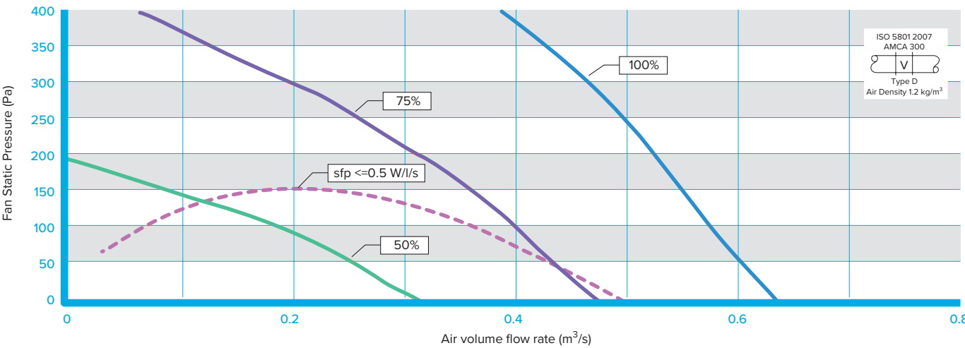
EXTRACT FAN SIZE DE5 - PERFORMANCE
